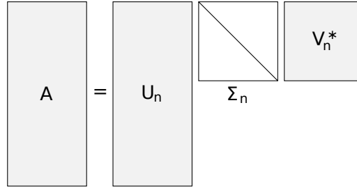
Fig. 1: Scheme of the thin SVD of a rectangular matrix A .
