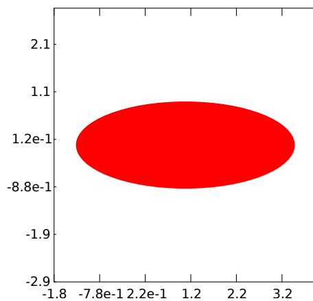
Fig. 3: Ellipse region defined via de RG class.
