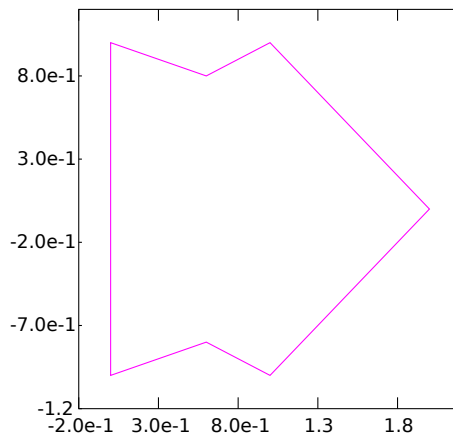
Fig. 2: Polygon region defined via de RG class.
