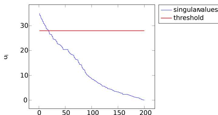
Fig. 3: Illustration of threshold usage with the singular values of the rdb200 matrix. The red line represents a threshold of \delta = 0.8 .
