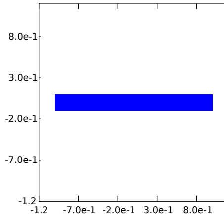
Fig. 1: Interval region defined via de RG class.
