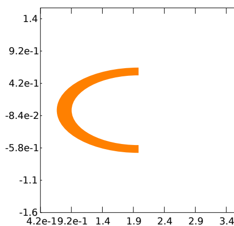
Fig. 4: Ring region defined via de RG class.
