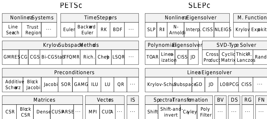
Fig. 1: Numerical components of PETSc and SLEPc
